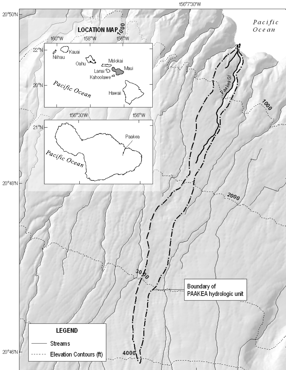
Figure 1-4. Elevation range and the location of Paakea hydrologic unit. (Source: State of Hawaii, Office of Planning, 1983; USGS, 2001b).
