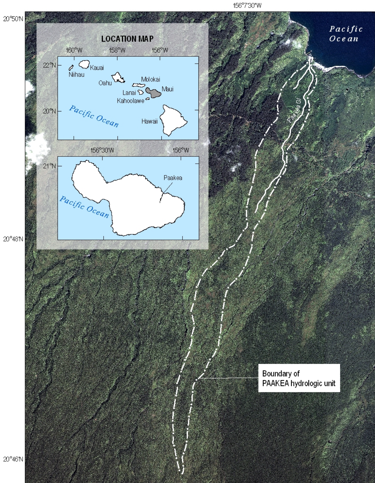
Figure 1-6. Quickbird satellite imagery of Paakea hydrologic unit (Source: County of Maui, Planning Department, 2004; USGS, 2001b).
