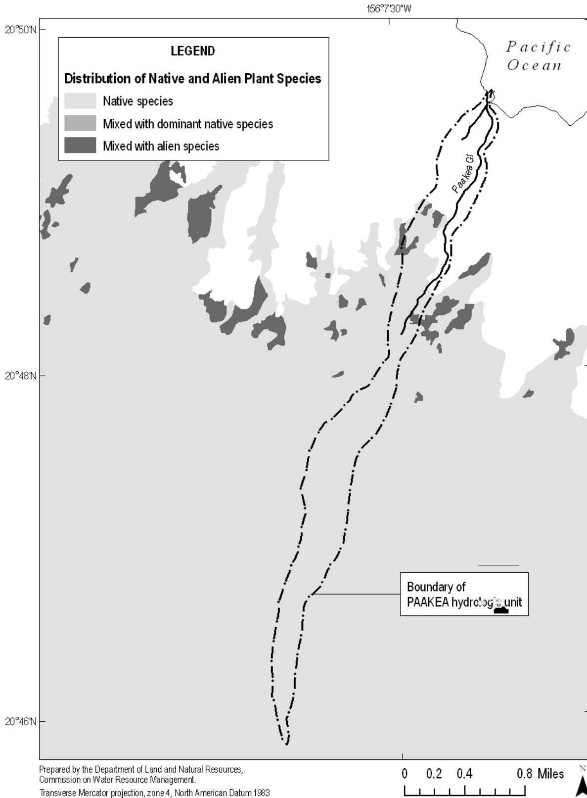
Figure 6-3. Distribution of native and alien plant species for Paakea hydrologic unit (Source: Jacobi, 1989; Scott et al., 1986; State of Hawaii, Office of Planning, 1992, 2004b; 2004d; USGS, 2001b).
