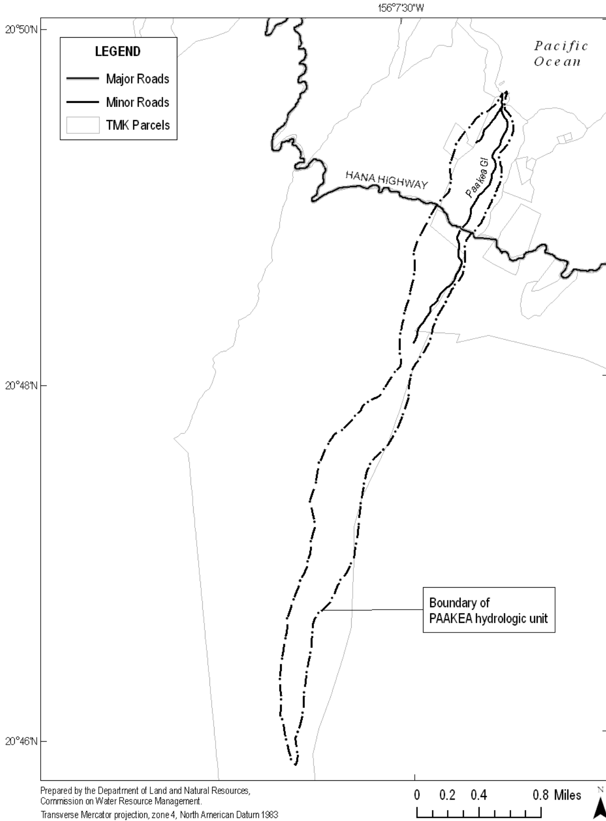
Figure 1-5. Major and minor roads and Tax Map Key (TMK) parcel boundaries for Paakea hydrologic unit (Source: County of Maui, 2006; County of Maui, Geographic Information Systems [GIS] Division, Department of Management, 2006; USGS, 2001b).
