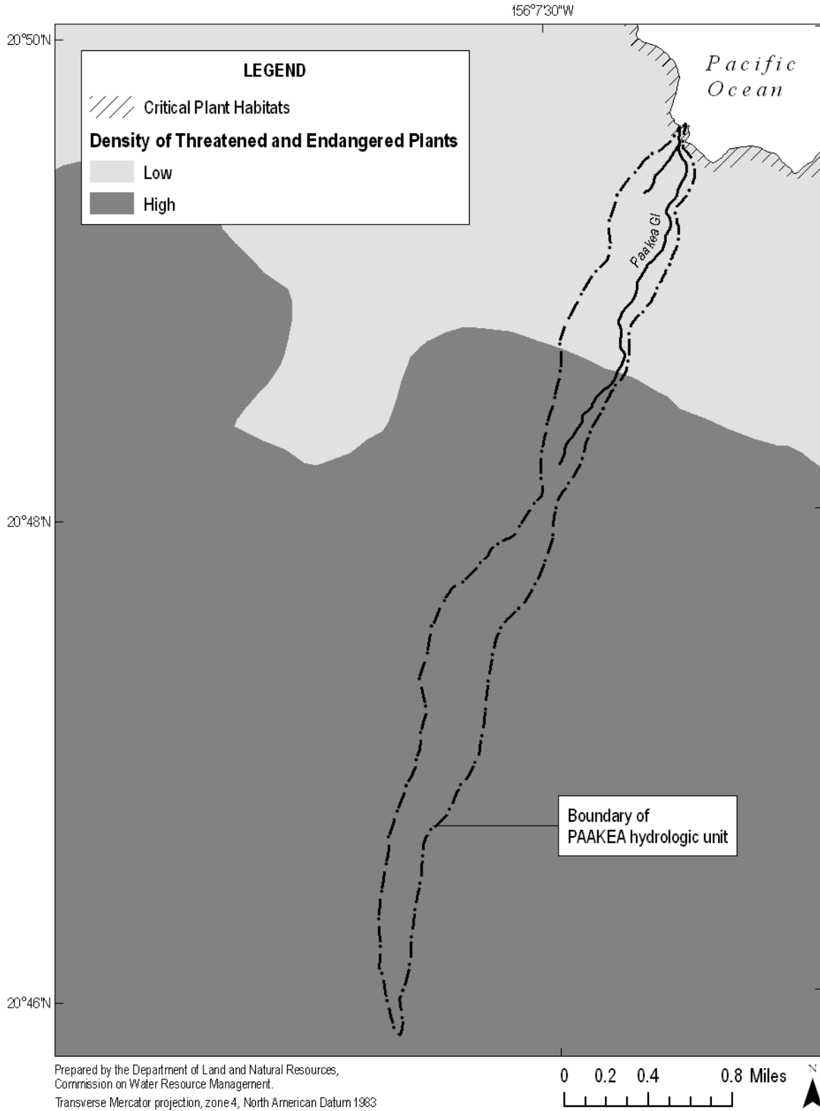
Figure 6-4. Critical plant habitats, and density of threatened and endangered plant species for Paakea hydrologic unit (Source: Jacobi, 1989; Scott et al., 1986; State of Hawaii, Office of Planning, 1992, 2004b; 2004d; USGS, 2001b).
