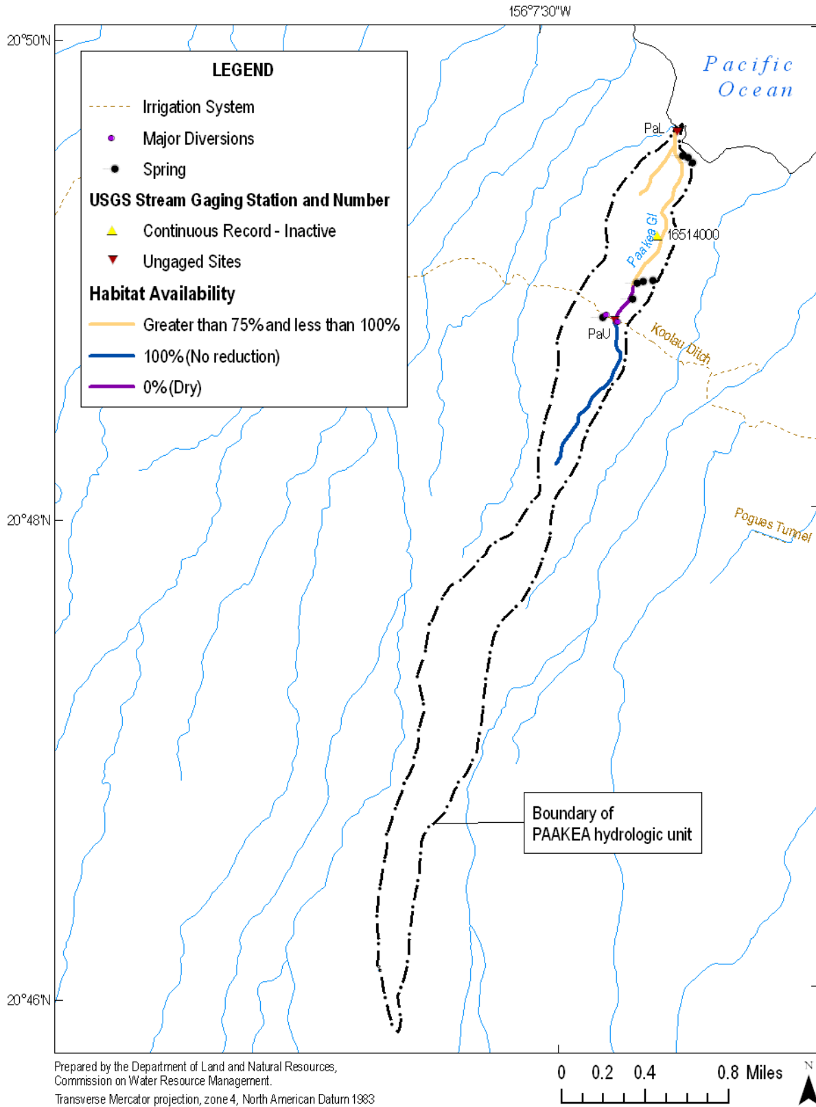
Figure 4-3. Estimated habitat availability in Paakea hydrologic unit (Source: Gingerich and Wolff, 2005; USGS, 2001b).
