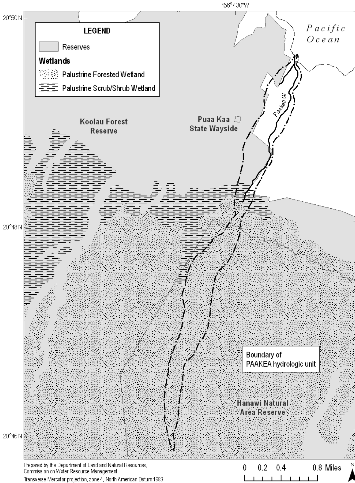
Figure 6-2. Reserves and wetlands for the Paakea hydrologic unit (Source: State of Hawaii, Office of Planning, 2003; 2007b; USGS, 2001b).
