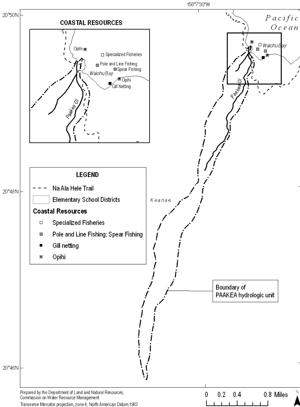
Figure 5-2. Recreational points of interest for Paakea hydrologic unit (Source: State of Hawaii, Office of Planning, 1999, 2002a; 2002c; 2002d; 2004a; USGS, 2001b).
