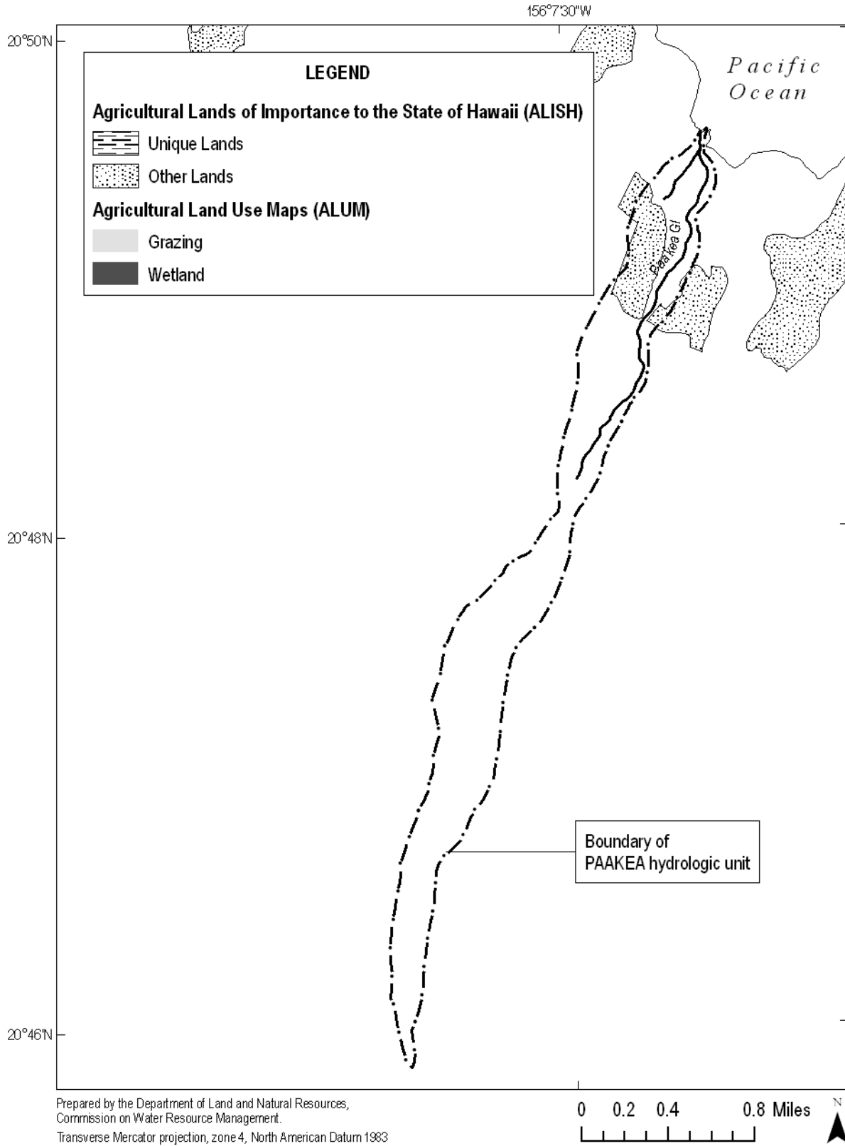
Figure 13-20. Potential agricultural land use for the Paakea hydrologic unit based on the ALISH and ALUM classification systems (Source: State of Hawaii, Office of Planning, 1977; 1980; USGS, 2001b).
