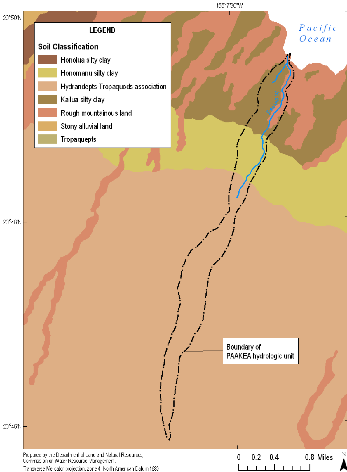
Figure 2-3. Soil classification in Paakea hydrologic unit (Source: State of Hawaii, Office of Planning, 2007c; USGS, 2001b).
