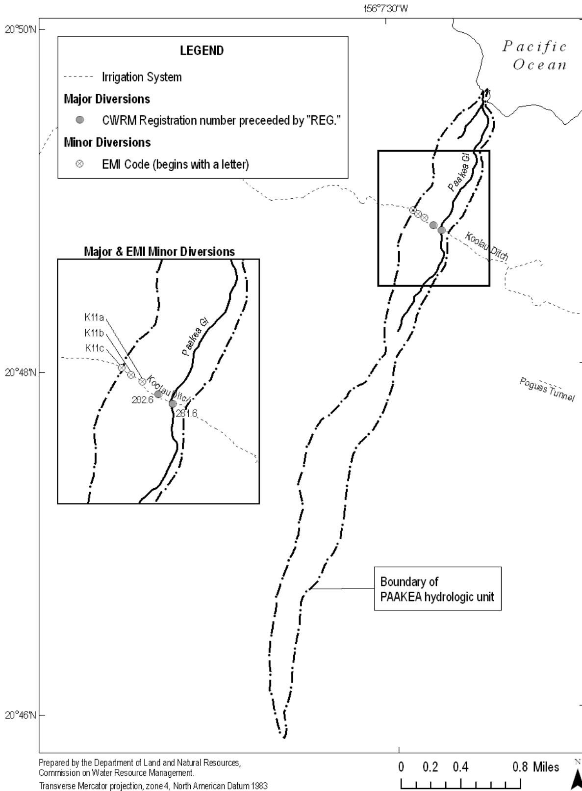
Figure 13-19. All registered diversions and EMI minor diversions identified in the Paakea hydrologic unit (Source: East Maui Irrigation Company, 1970; State of Hawaii, Commission on Water Resource Management, 2008f; USGS, 2001b).
