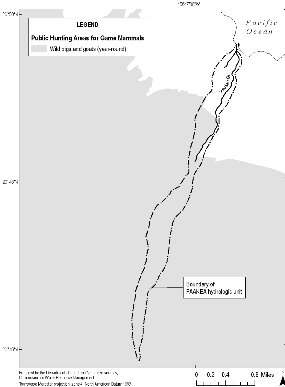
Figure 5-1. Public hunting areas for game mammals in Paakea hydrologic unit (Source: State of Hawaii, Office of Planning, 2002b; USGS, 2001b).
