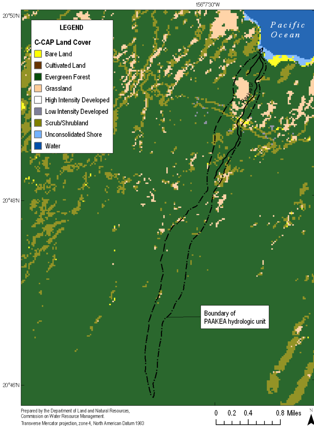
Figure 2-6. C-CAP land cover in Paakea hydrologic unit (Source: National Oceanic and Atmospheric Administration, Coastal Services Center, 2000; USGS, 2001b).
